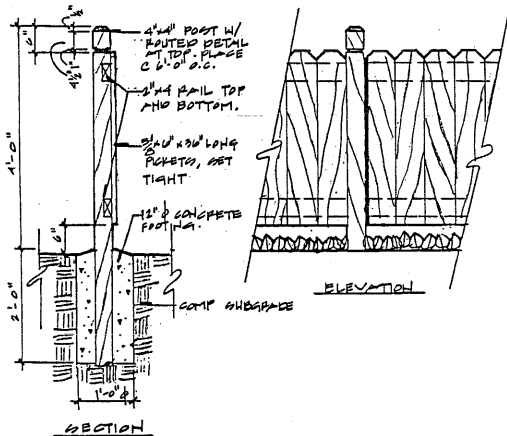
FRONT AND SIDE YARD FENCE DETAIL
