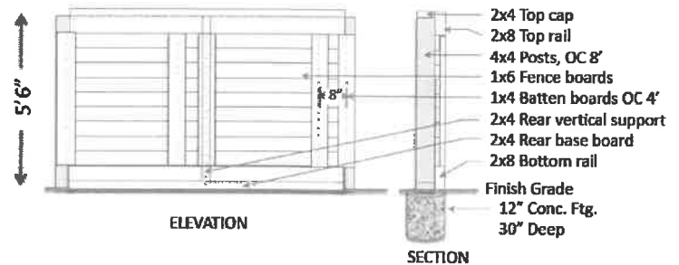
Alden Park Prototypical Design for Fences Facing Public Street
